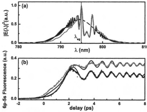
Figure 10.10. Realization of a temporal Fresnel lens with a low resolution pulse shaper. (a) Calculated (black) and realized (grey) spectra. Original spectrum (dashed line). \lambda_{eg} = 794.95 nm. (b) Transient population measurements (dots) and numerical solution (line) obtained with the experimental spectrum (grey), together with the normal CT (black). Here, \phi'' = -4.9 \cdot 10^5 fs 2 corresponding to \tau_c \simeq 12.4 ps [28].
