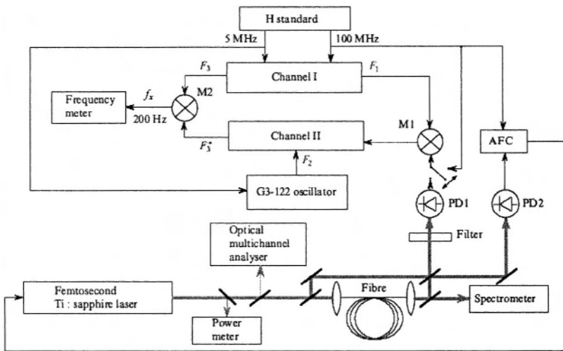
Figure 4-8. Principal scheme of the experimental set-up. AFC: automatic frequency control; M1, M2: mixers; PD1, PD2: photodiodes.
